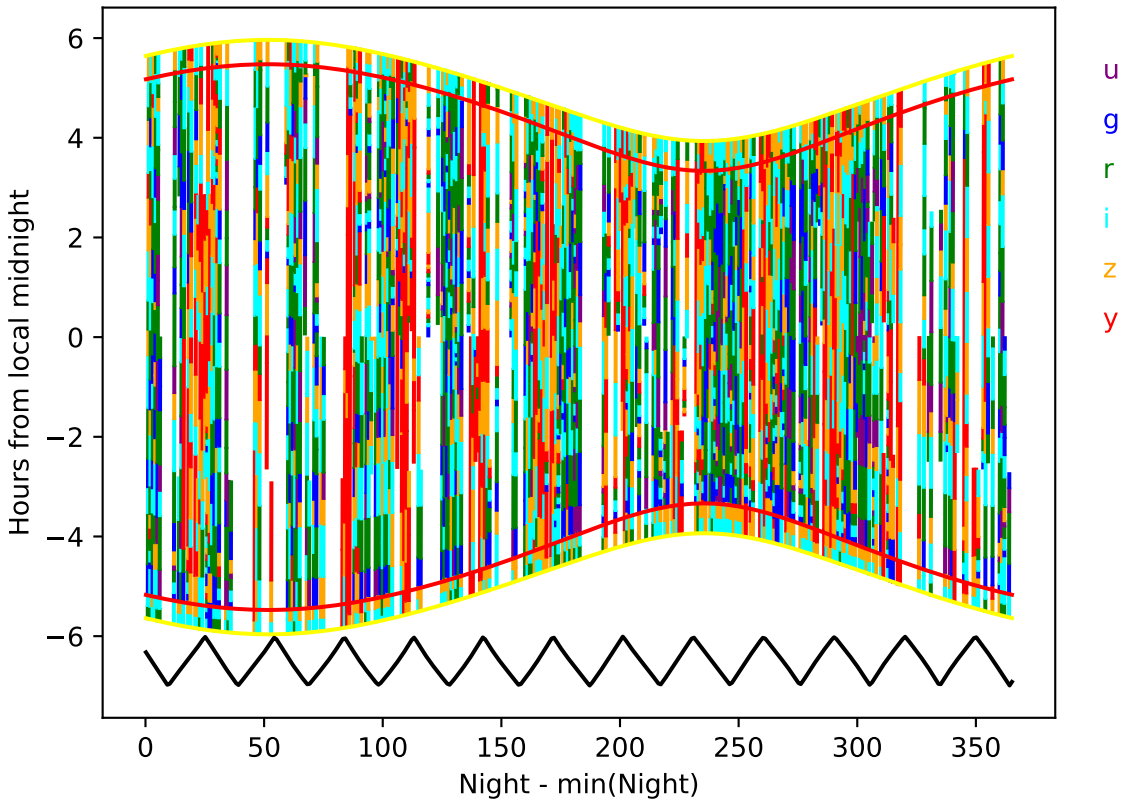
too_elab_r8_d3_ugrizy_v3.4_10yrs year 7-8: Hourglass
