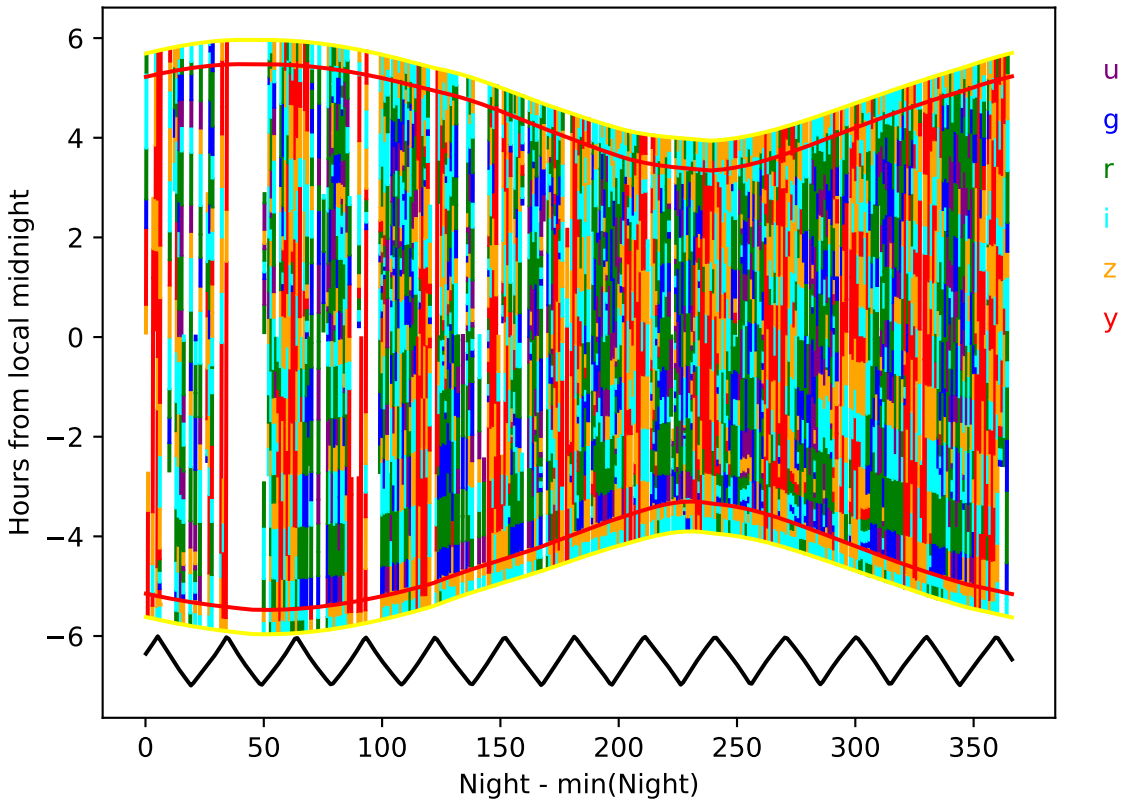
too_elab_r8_d3_ugrizy_v3.4_10yrs year 6-7: Hourglass
