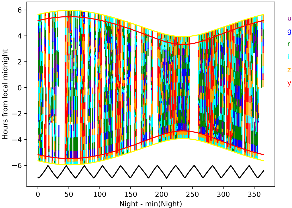
too_elab_r8_d3_ugrizy_v3.4_10yrs year 5-6: Hourglass
