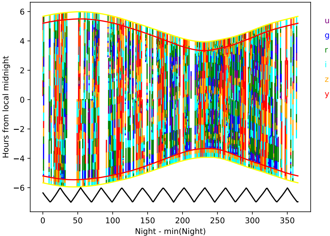
too_elab_r8_d3_ugrizy_v3.4_10yrs year 4-5: Hourglass
