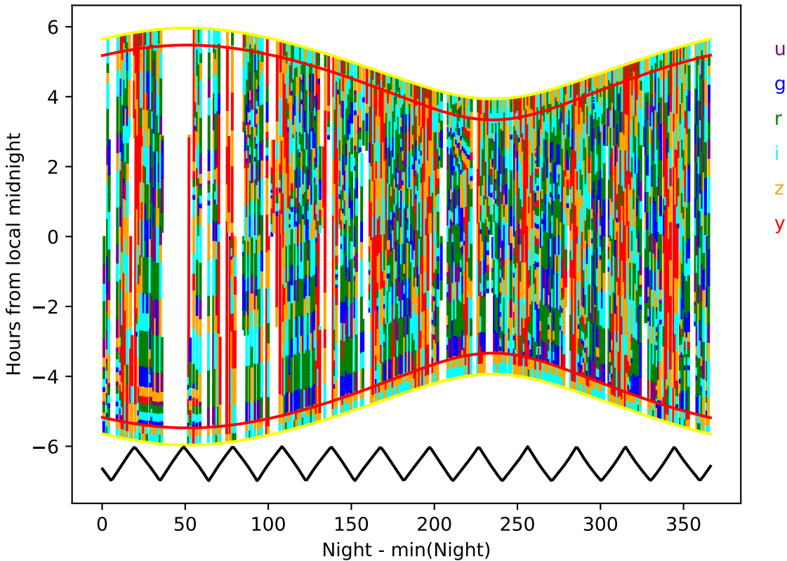
too_elab_r8_d3_ugrizy_v3.4_10yrs year 2-3: Hourglass
