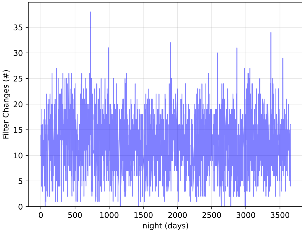
too_elab_r8_d3_ugrizy_v3.4_10yrs : Filter Changes
