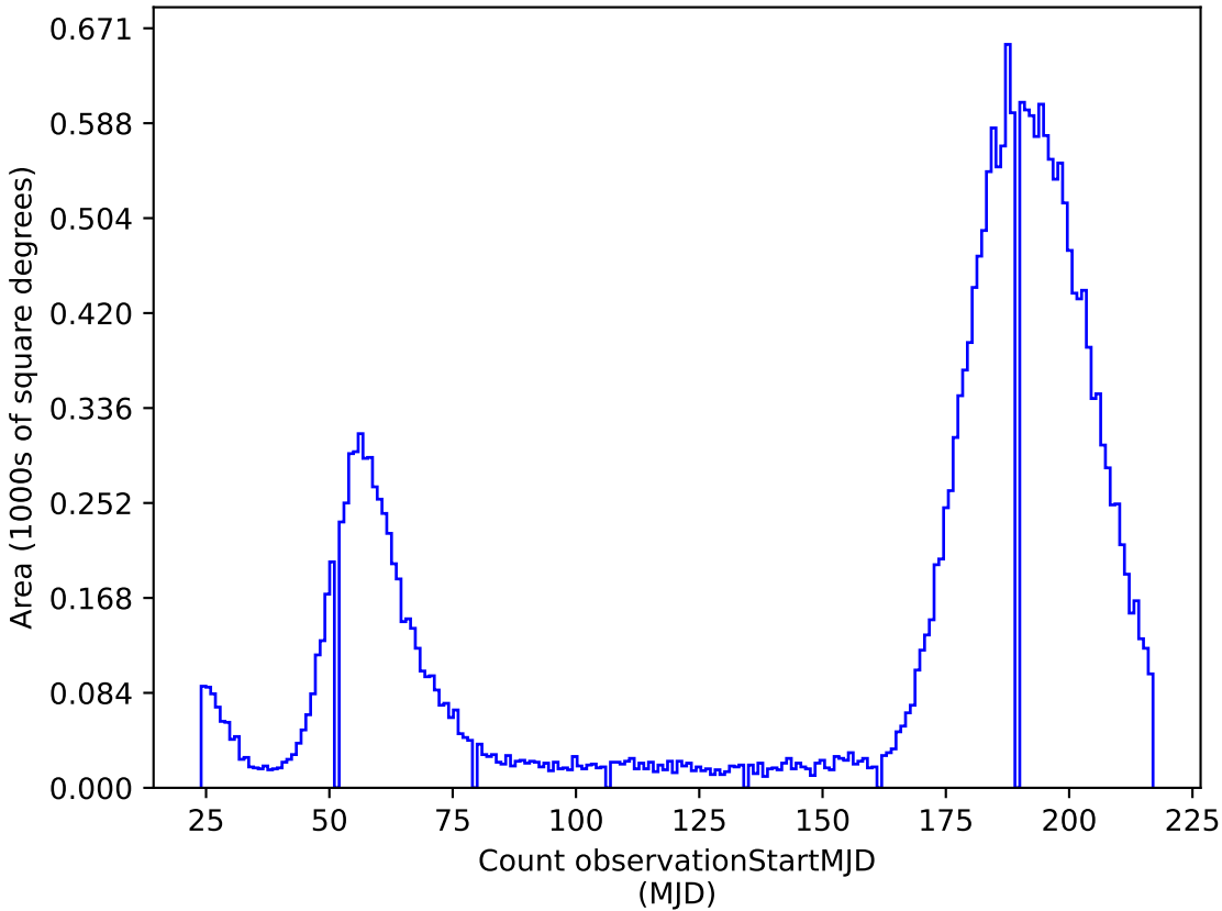
too_elab_r8_d3_ugrizy_v3.4_10yrs i: Count observationStartMJD
