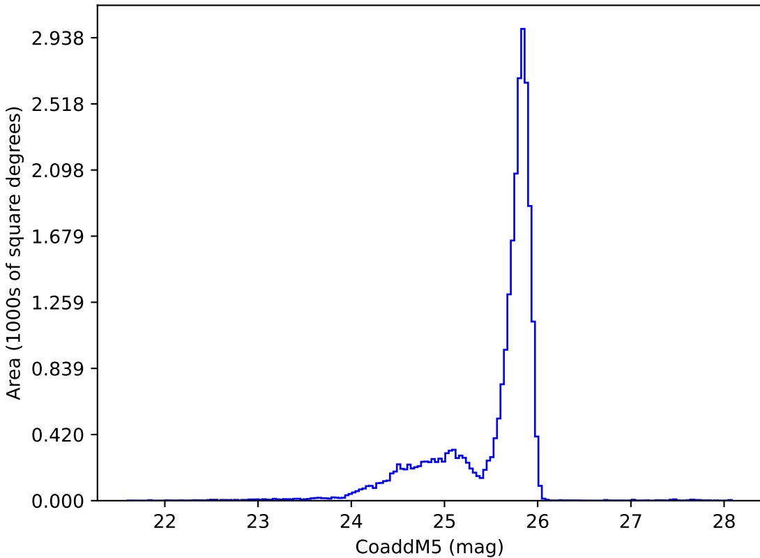
too_elab_r8_d3_ugrizy_v3.4_10yrs z: CoaddM5
