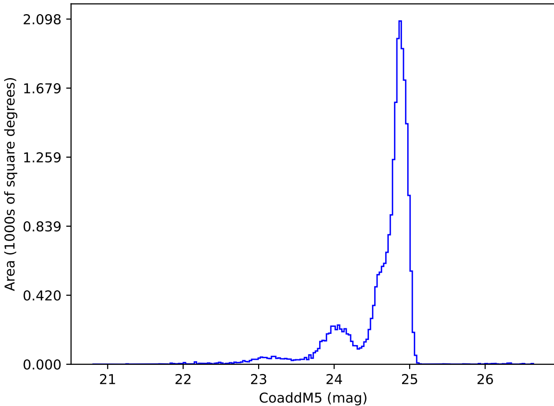
too_elab_r8_d3_ugrizy_v3.4_10yrs y: CoaddM5
