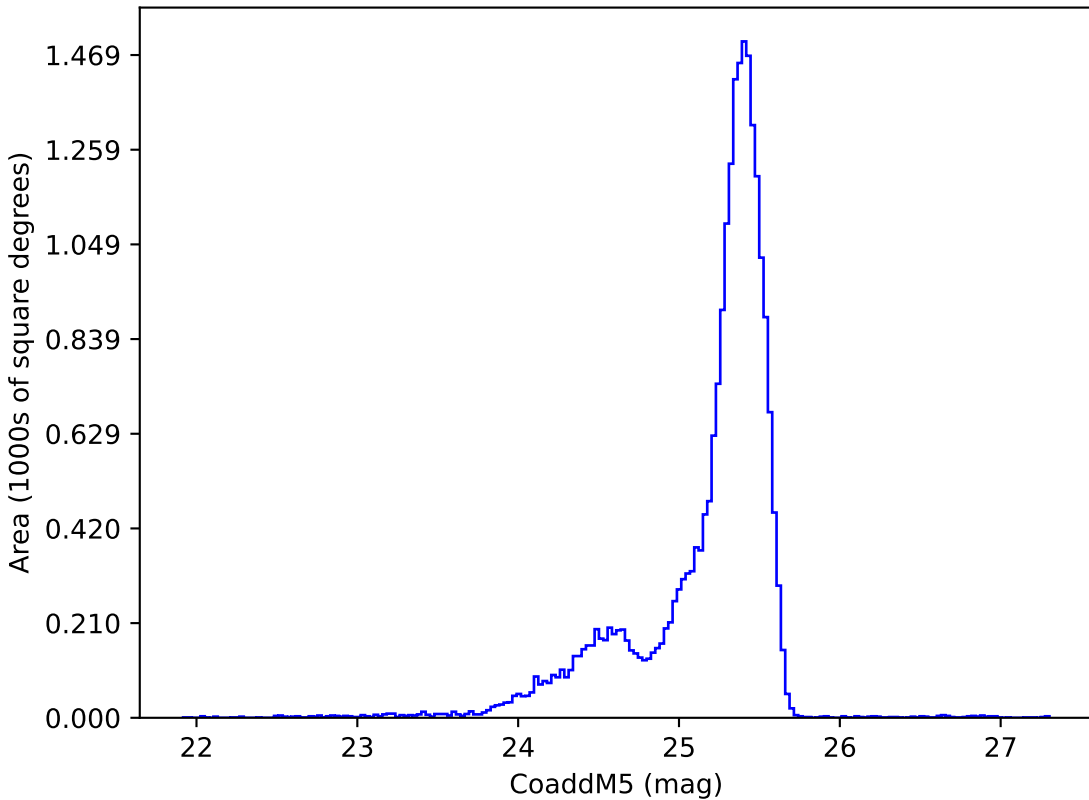
too_elab_r8_d3_ugrizy_v3.4_10yrs u: CoaddM5
