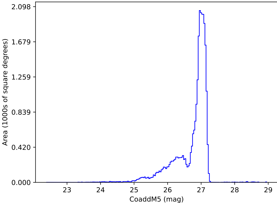
too_elab_r8_d3_ugrizy_v3.4_10yrs r: CoaddM5
