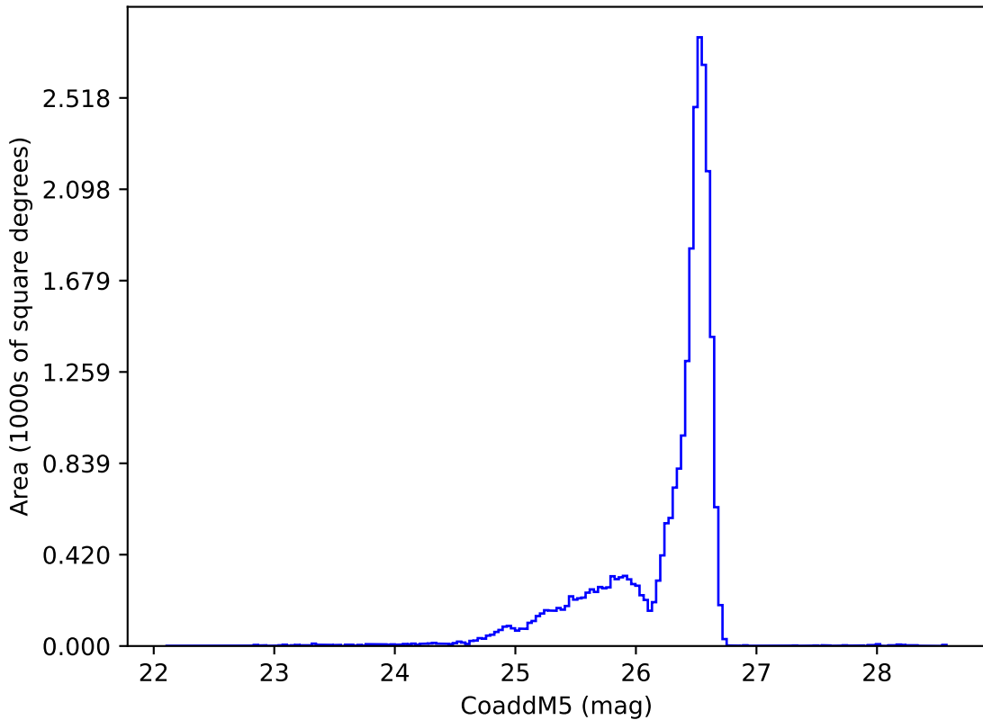
too_elab_r8_d3_ugrizy_v3.4_10yrs i: CoaddM5
