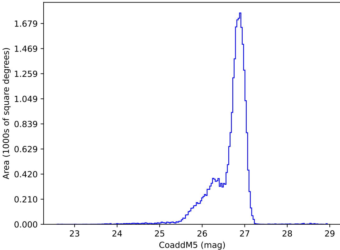
too_elab_r8_d3_ugrizy_v3.4_10yrs g: CoaddM5
