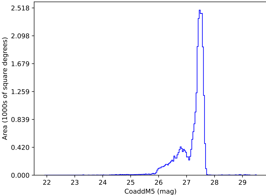
too_elab_r8_d3_ugrizy_v3.4_10yrs : CoaddM5
