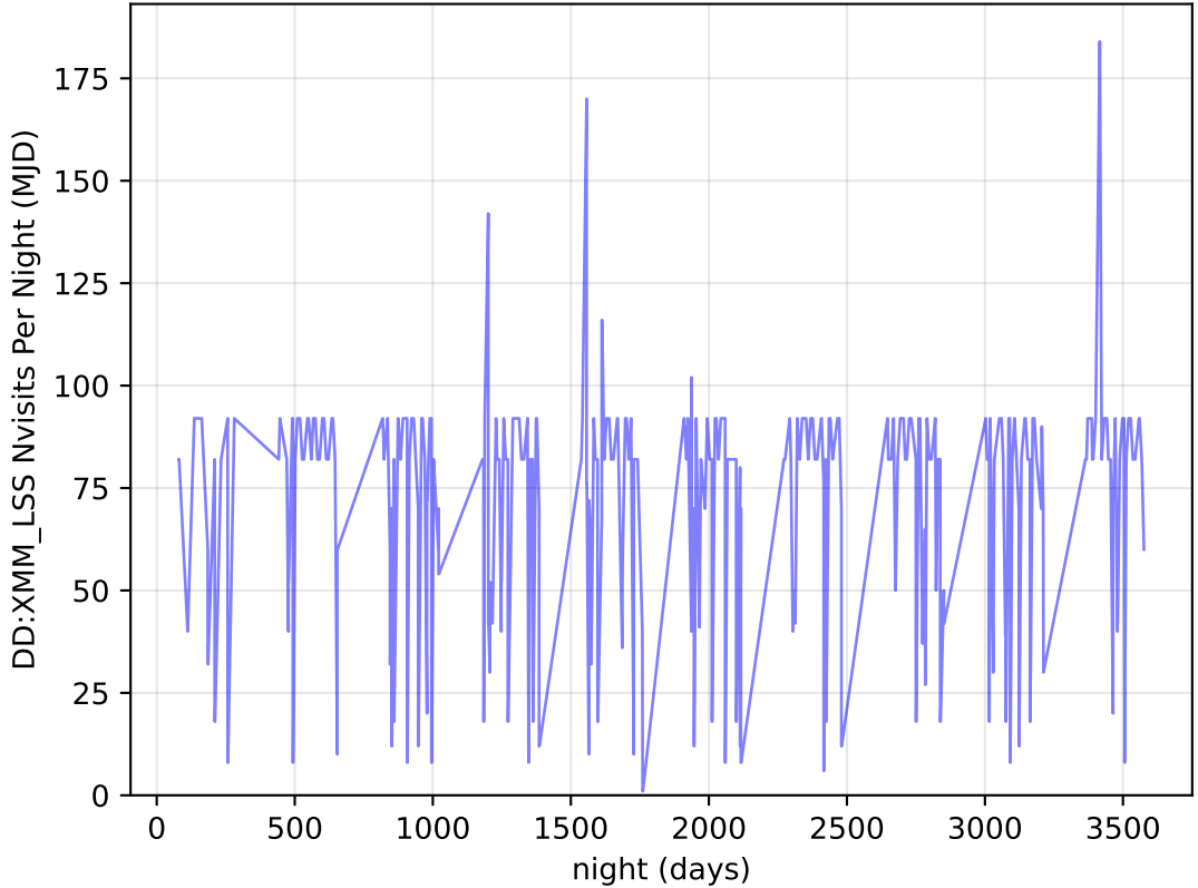
too_elab_r8_d3_ugrizy_v3.4_10yrs all bands: DD:XMM_LSS Nvisits Per Night
