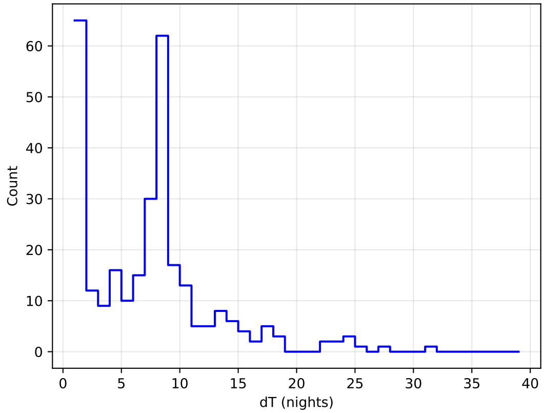
too_elab_r8_d3_ugrizy_v3.4_10yrs all bands: DD:XMM_LSS Delta Nights Histogram
