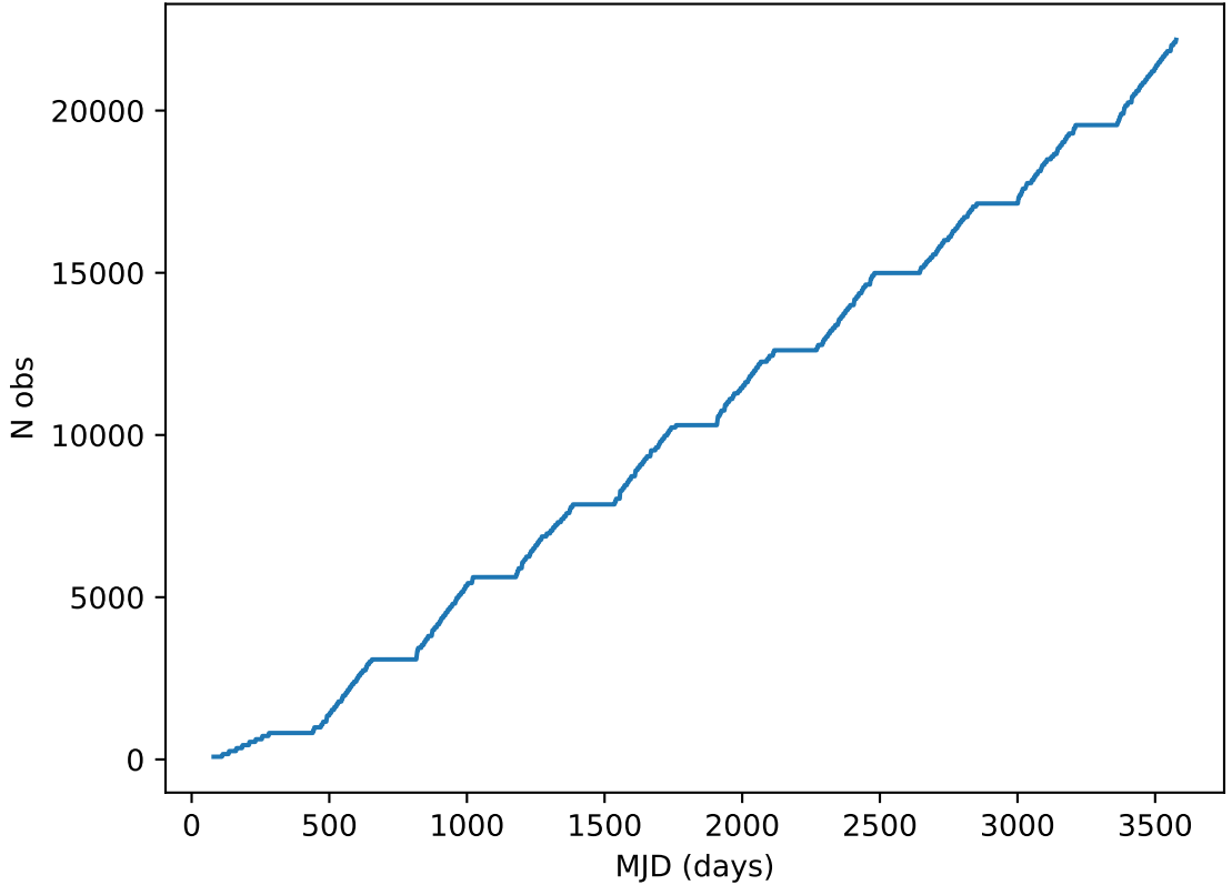
too_elab_r8_d3_ugrizy_v3.4_10yrs all bands: DD:XMM_LSS Cumulative NVisits
