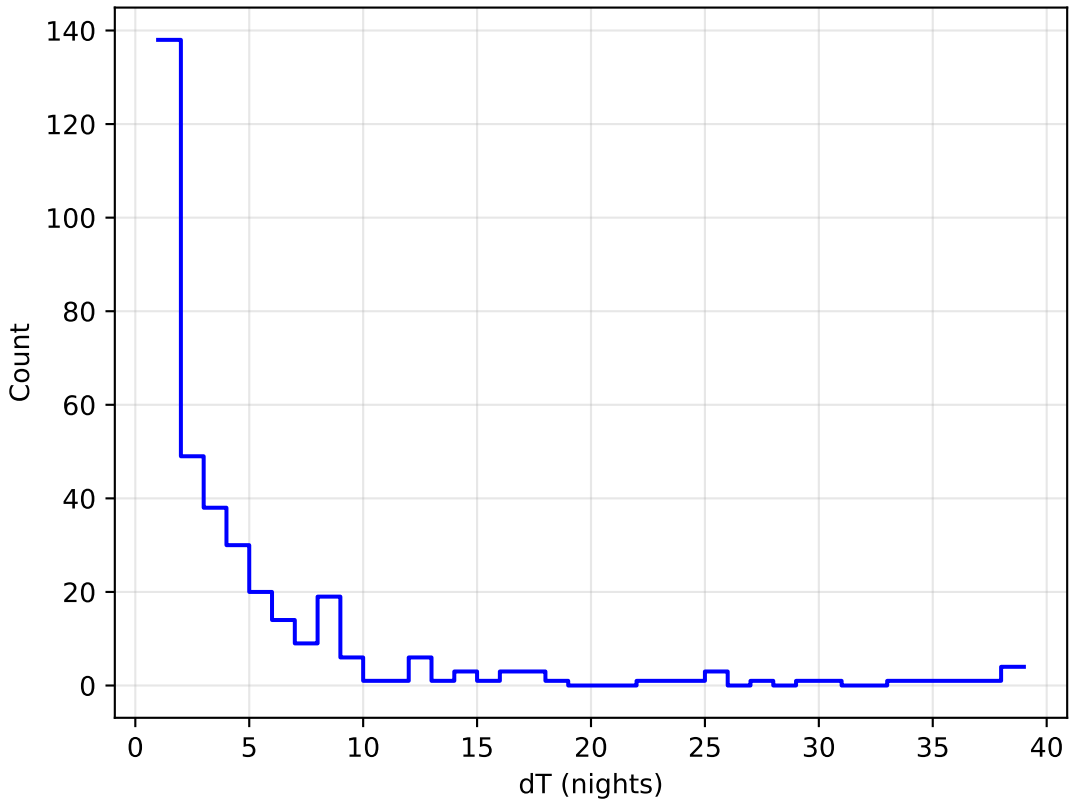
too_elab_r8_d3_ugrizy_v3.4_10yrs all bands: DD:WFD Delta Nights Histogram
