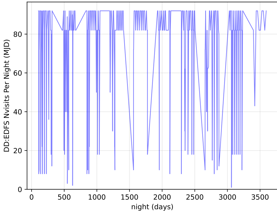
too_elab_r8_d3_ugrizy_v3.4_10yrs all bands: DD:EDFS Nvisits Per Night
