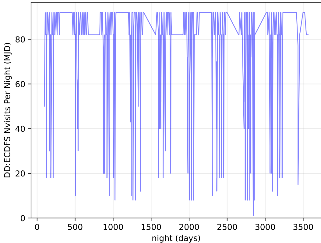
too_elab_r8_d3_ugrizy_v3.4_10yrs all bands: DD:ECDFS Nvisits Per Night
