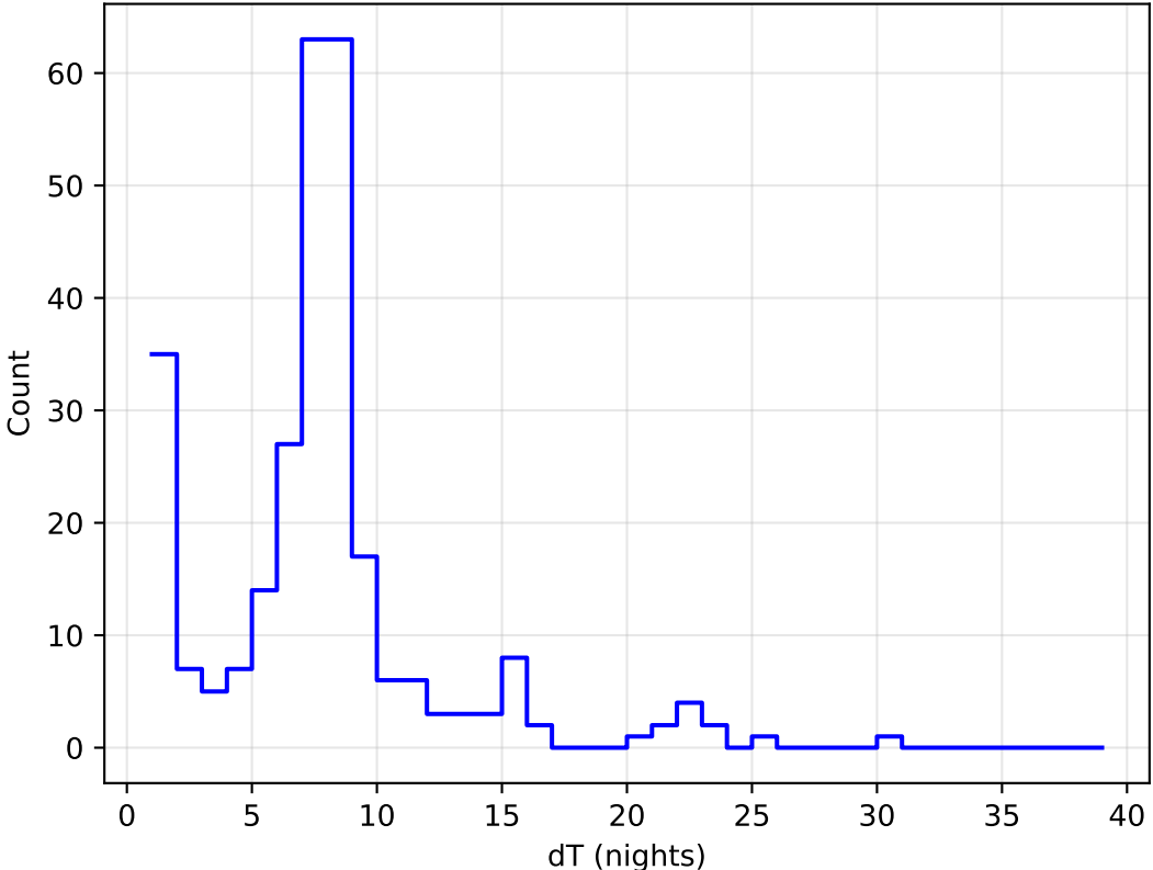
too_elab_r8_d3_ugrizy_v3.4_10yrs all bands: DD:ECDFS Delta Nights Histogram
