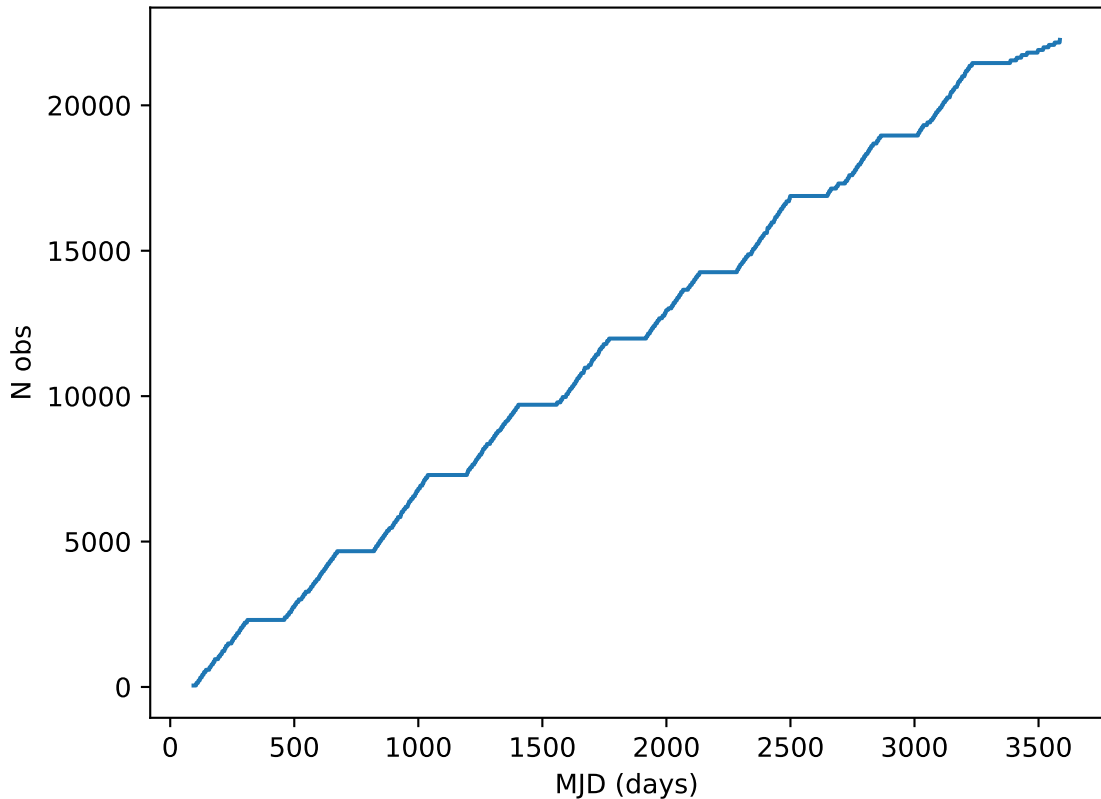
too_elab_r8_d3_ugrizy_v3.4_10yrs all bands: DD:ECDFS Cumulative NVisits
