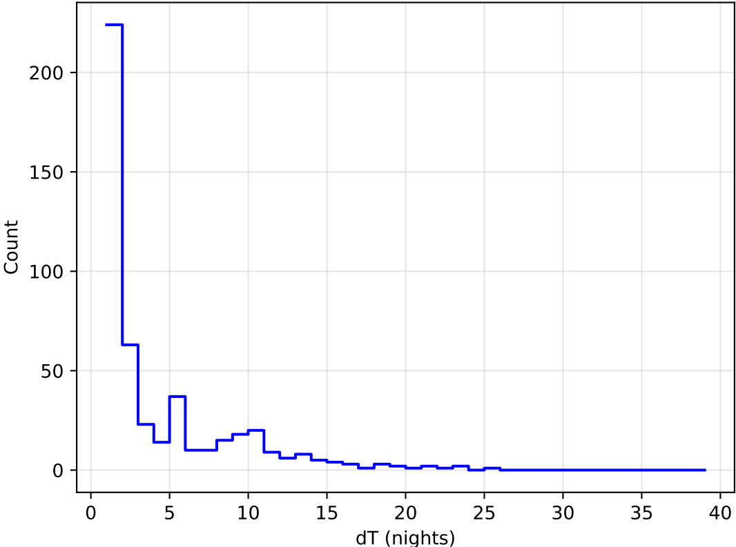
too_elab_r8_d3_ugrizy_v3.4_10yrs all bands: DD:COSMOS Delta Nights Histogram
