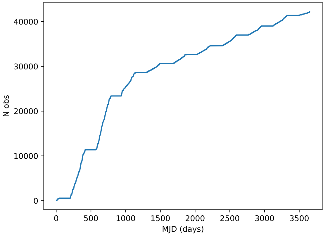
too_elab_r8_d3_ugrizy_v3.4_10yrs all bands: DD: COSMOS Cumulative NVisits
