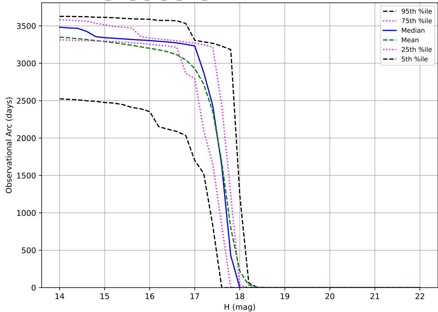
too_elab_r8_d3_gz_v3.4_10yrs: Observational Arc Length Trojan
