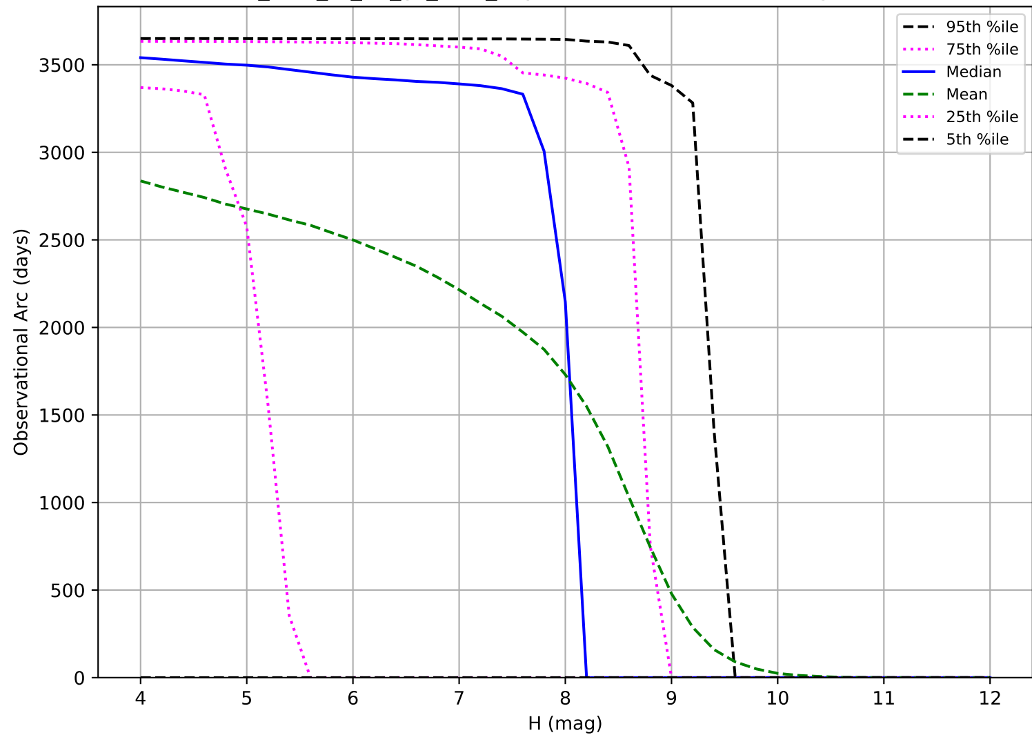
too_elab_r8_d3_gz_v3.4_10yrs: Observational Arc Length TNO
