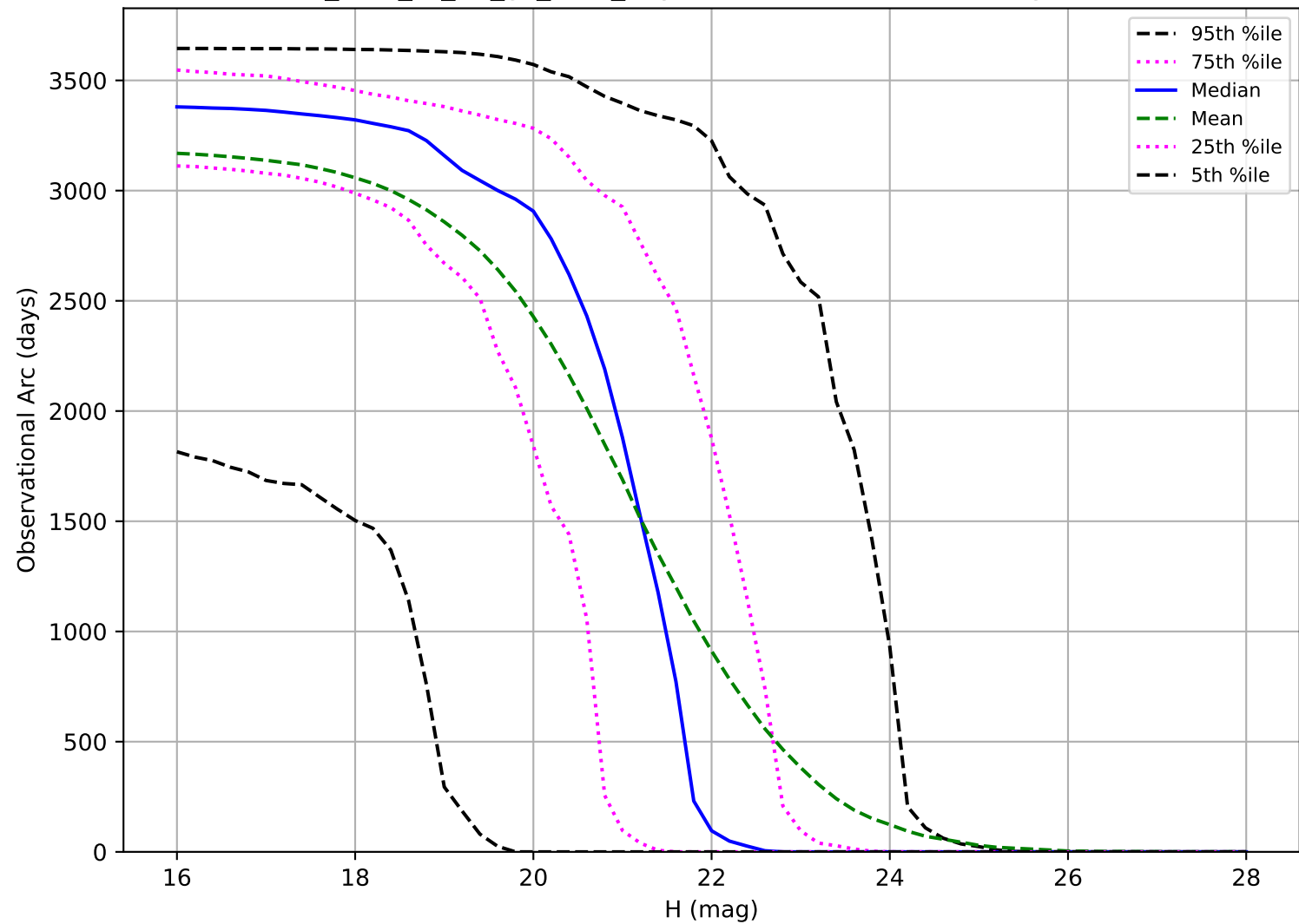
too_elab_r8_d3_gz_v3.4_10yrs: Observational Arc Length NEO
