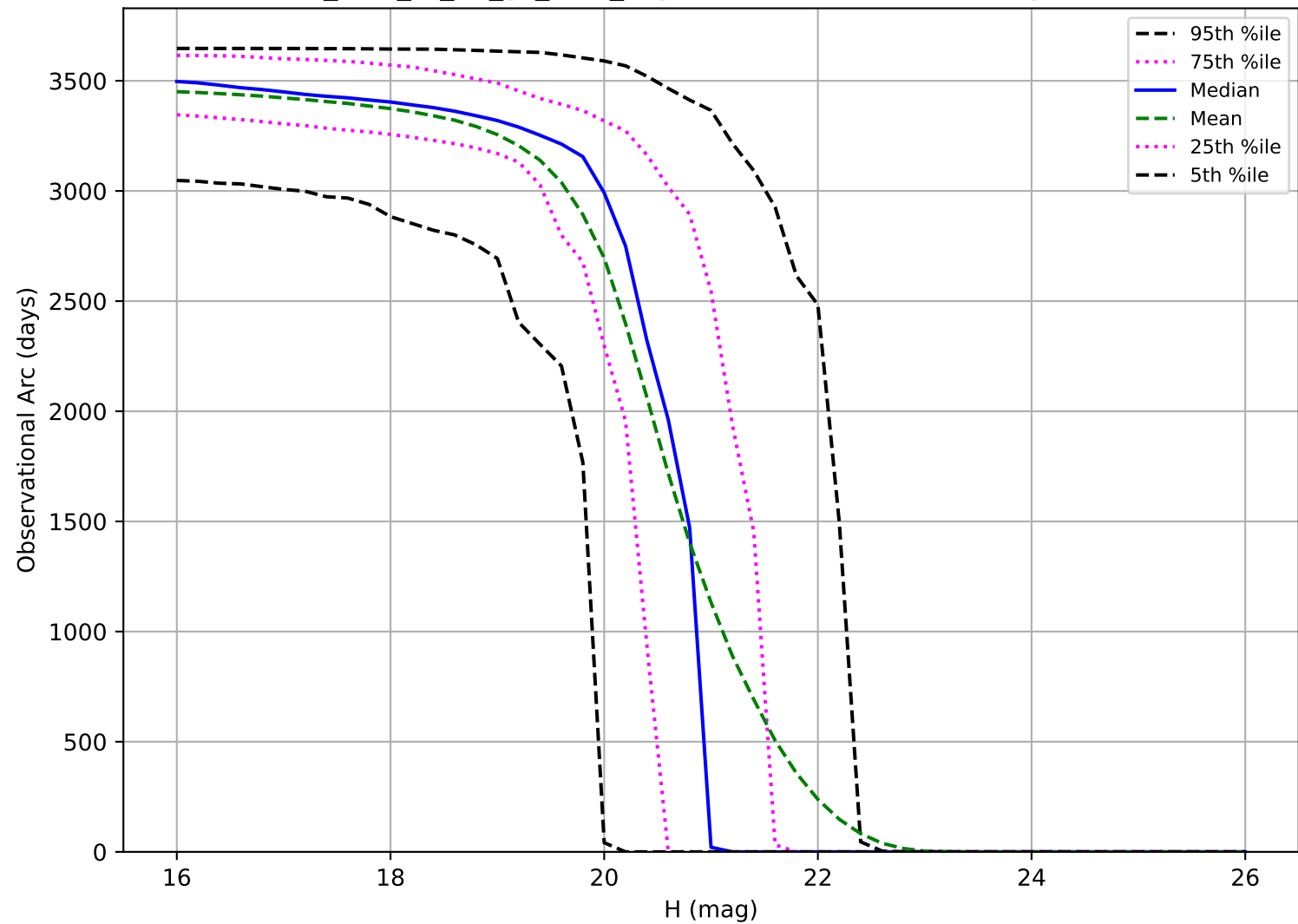
too_elab_r8_d3_gz_v3.4_10yrs: Observational Arc Length MBA
