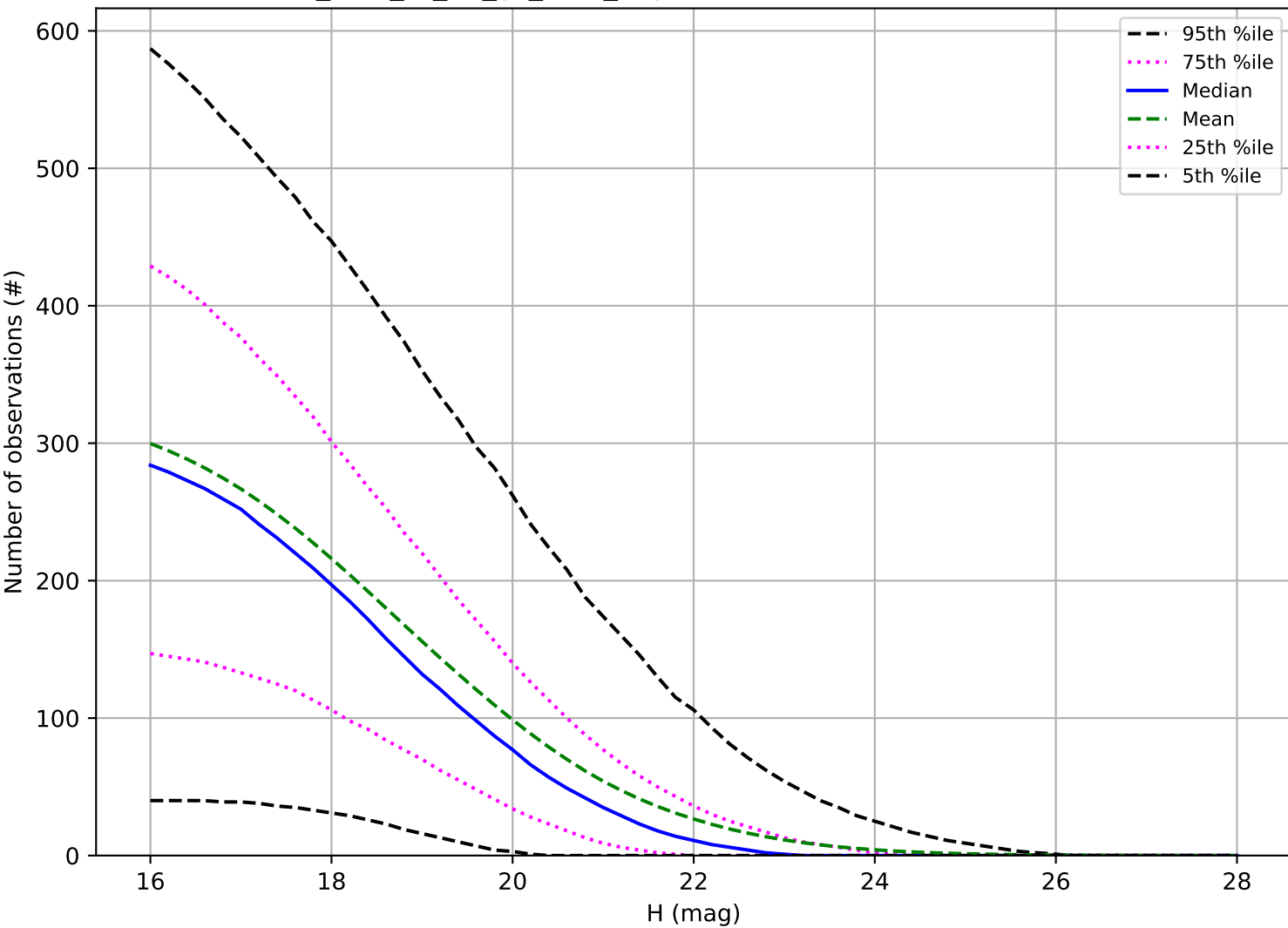
too_elab_r8_d3_gz_v3.4_10yrs: Number of observations PHA
