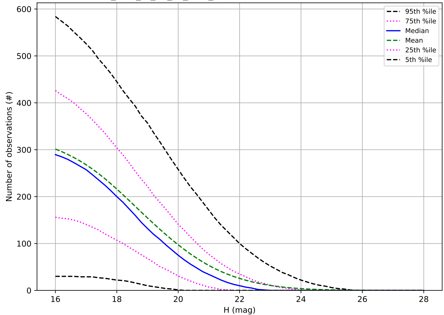
too_elab_r8_d3_gz_v3.4_10yrs: Number of observations NEO
