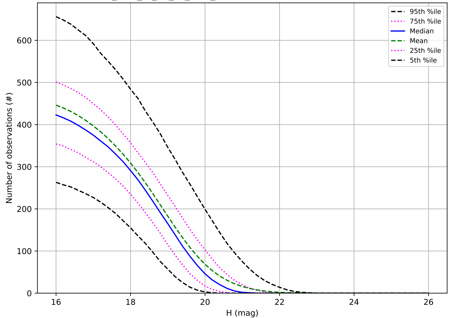
too_elab_r8_d3_gz_v3.4_10yrs: Number of observations MBA
