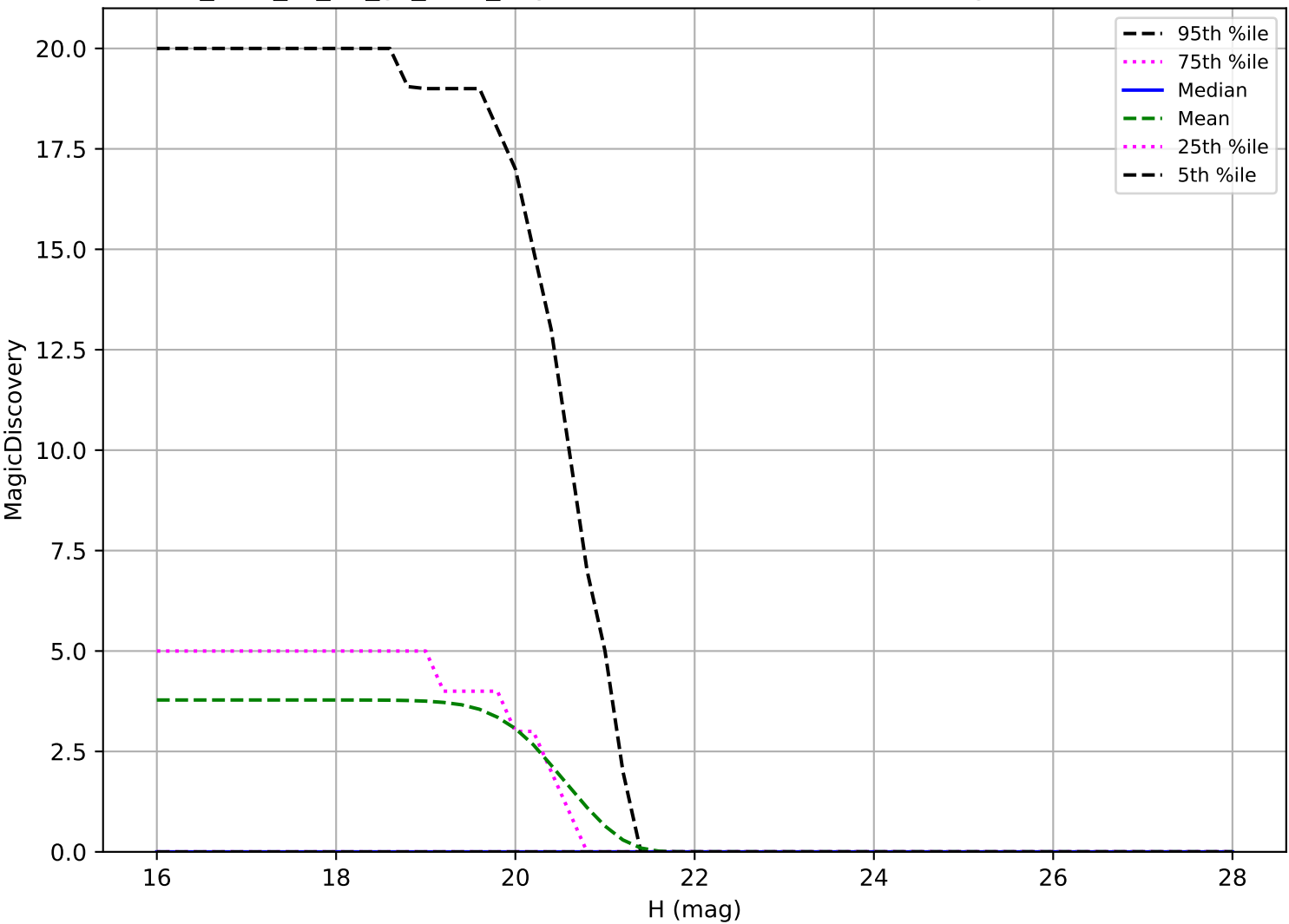
too_elab_r8_d3_gz_v3.4_10yrs: Vatira 6 detections in 60 nights detection loss
