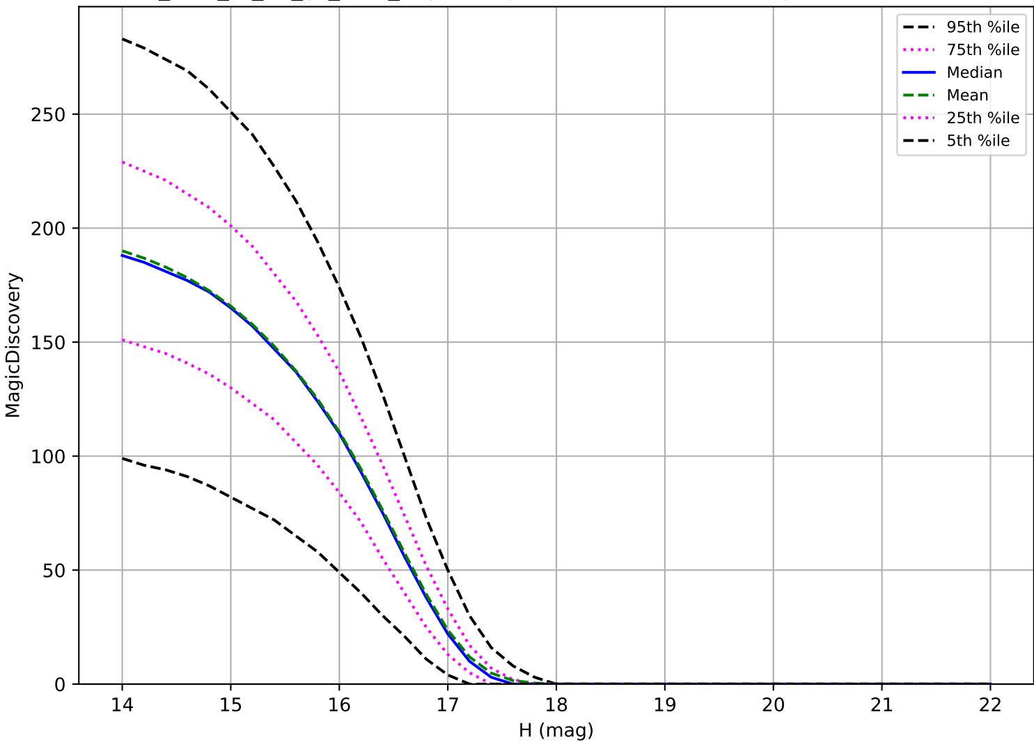
too_elab_r8_d3_gz_v3.4_10yrs: Trojan 6 detections in 60 nights detection loss
