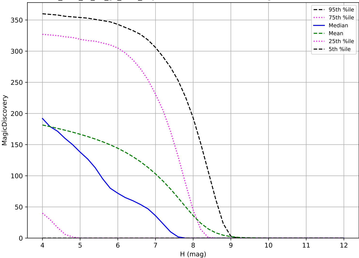
too_elab_r8_d3_gz_v3.4_10yrs: TNO 6 detections in 60 nights detection loss
