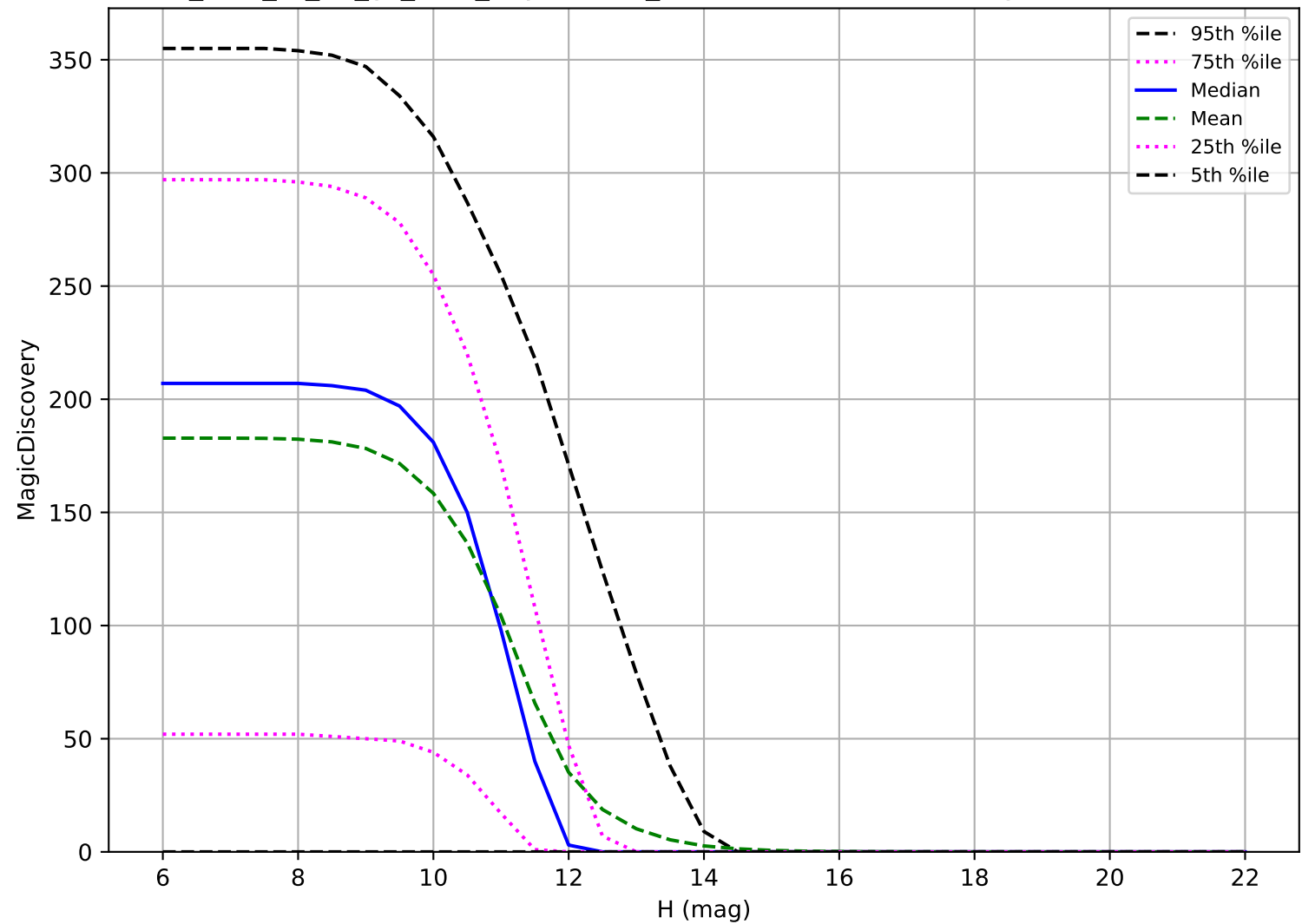
too_elab_r8_d3_gz_v3.4_10yrs: OCC_r20 6 detections in 60 nights detection loss
