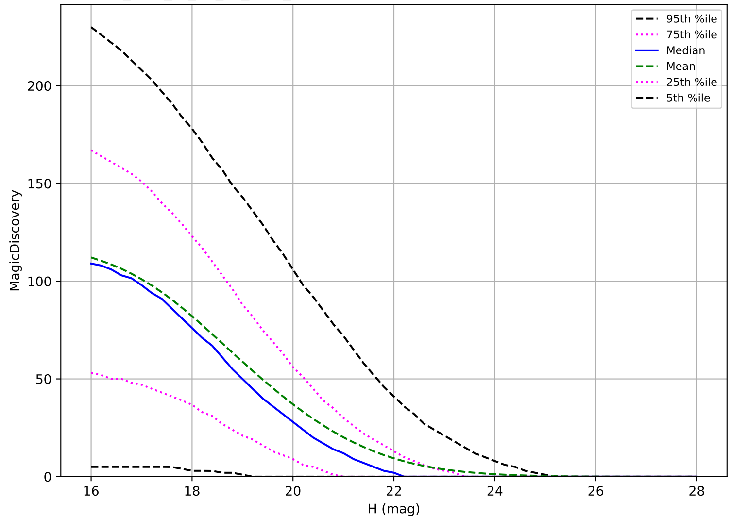
too_elab_r8_d3_gz_v3.4_10yrs: NEO 6 detections in 60 nights detection loss
