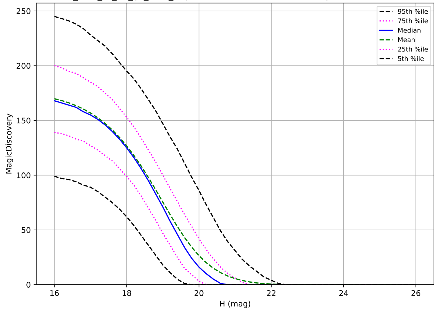
too_elab_r8_d3_gz_v3.4_10yrs: MBA 6 detections in 60 nights detection loss
