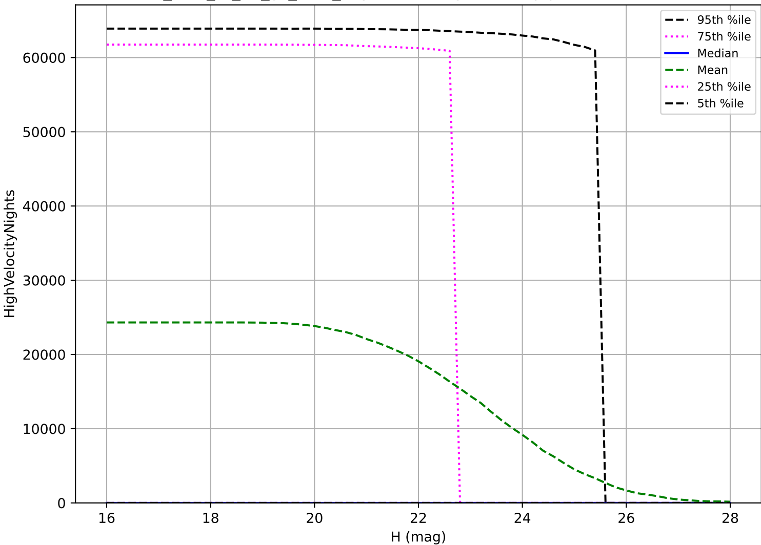
too_elab_r8_d3_gz_v3.4_10yrs: PHA High velocity pair detection loss
