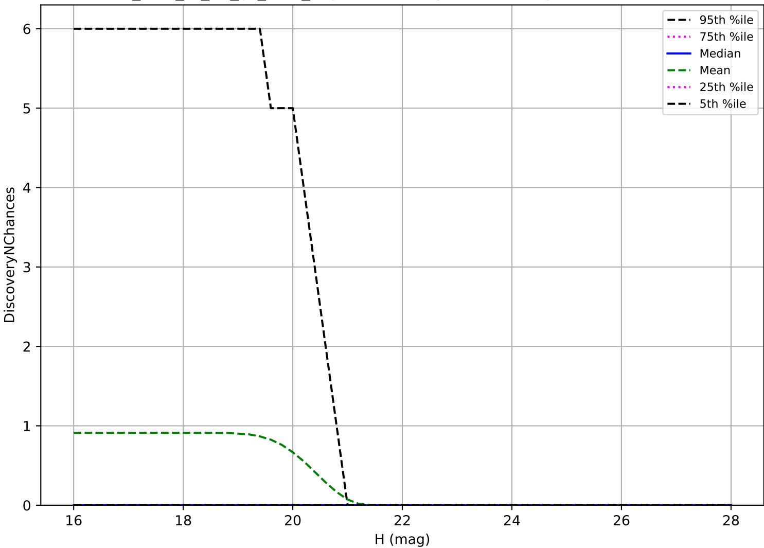
too_elab_r8_d3_gz_v3.4_10yrs: Vatira 3 pairs in 15 nights detection loss
