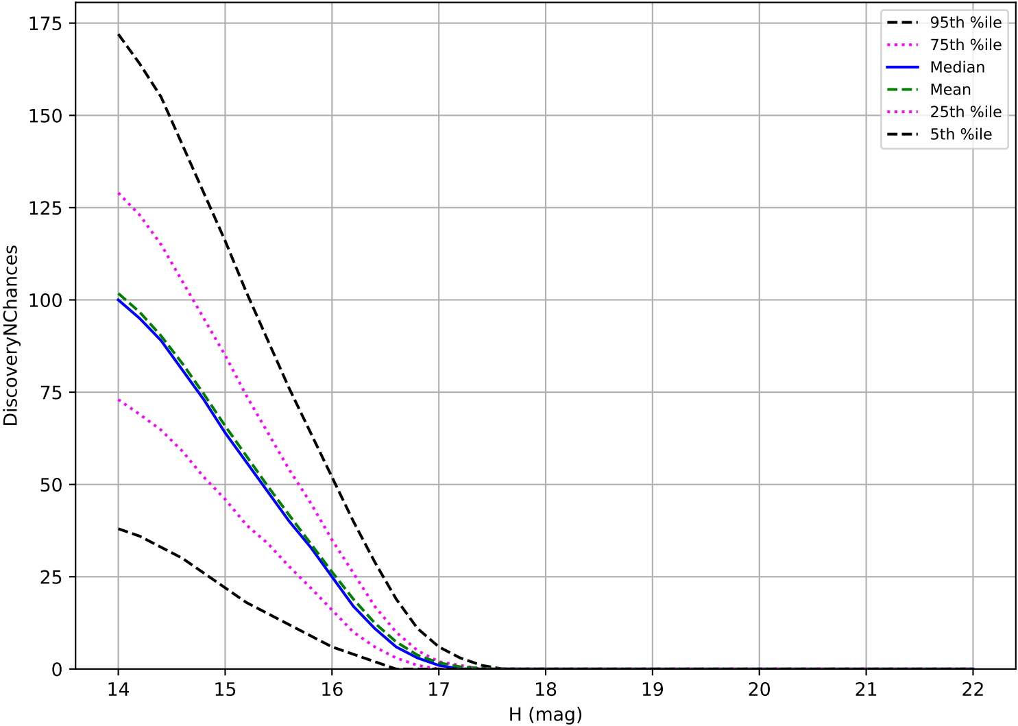
too_elab_r8_d3_gz_v3.4_10yrs: Trojan 3 pairs in 15 nights detection loss
