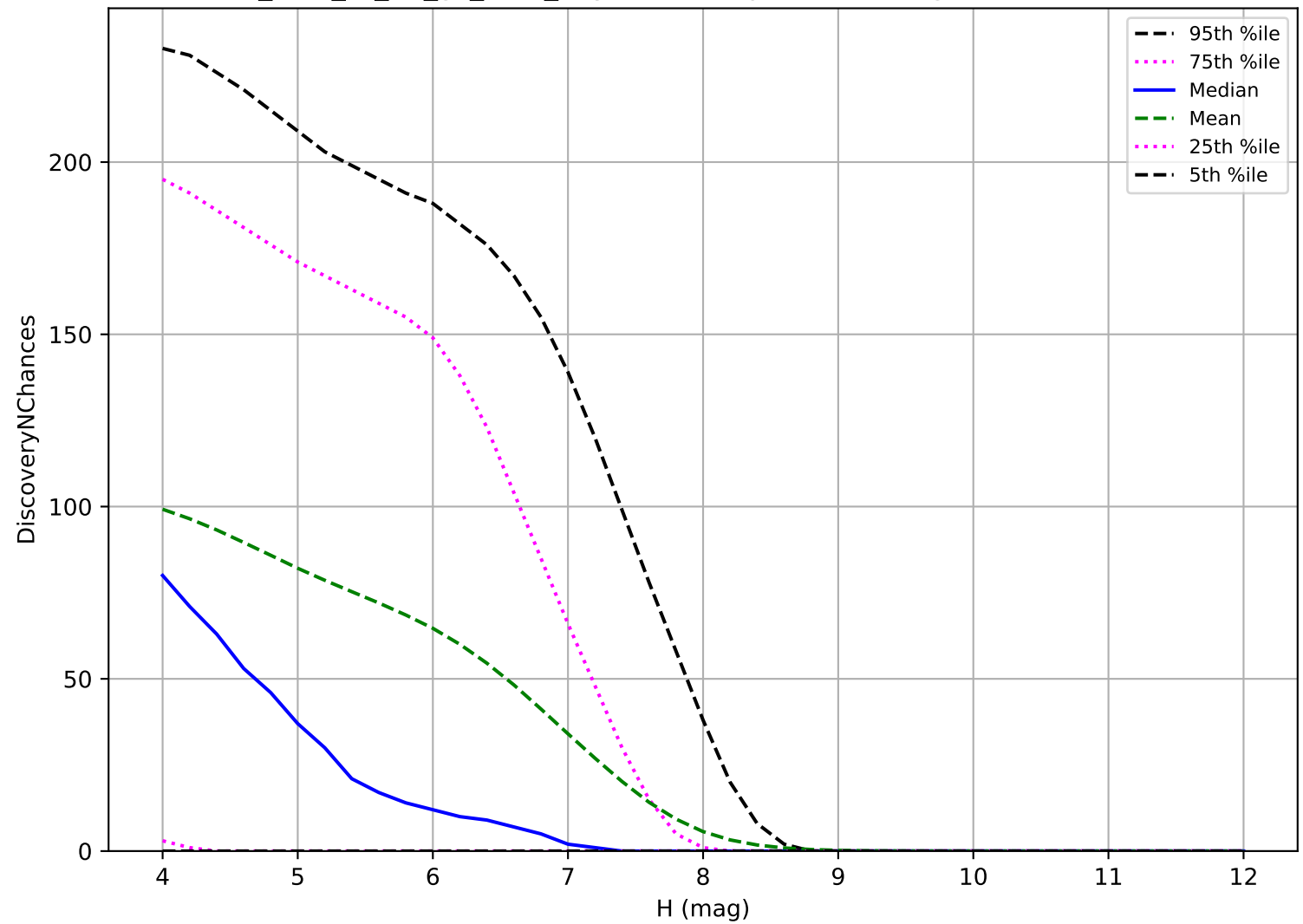
too_elab_r8_d3_gz_v3.4_10yrs: TNO 3 pairs in 15 nights detection loss
