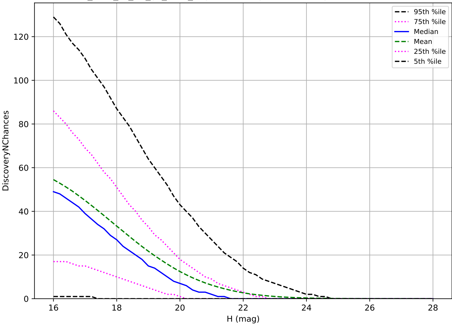
too_elab_r8_d3_gz_v3.4_10yrs: PHA 3 pairs in 15 nights detection loss
