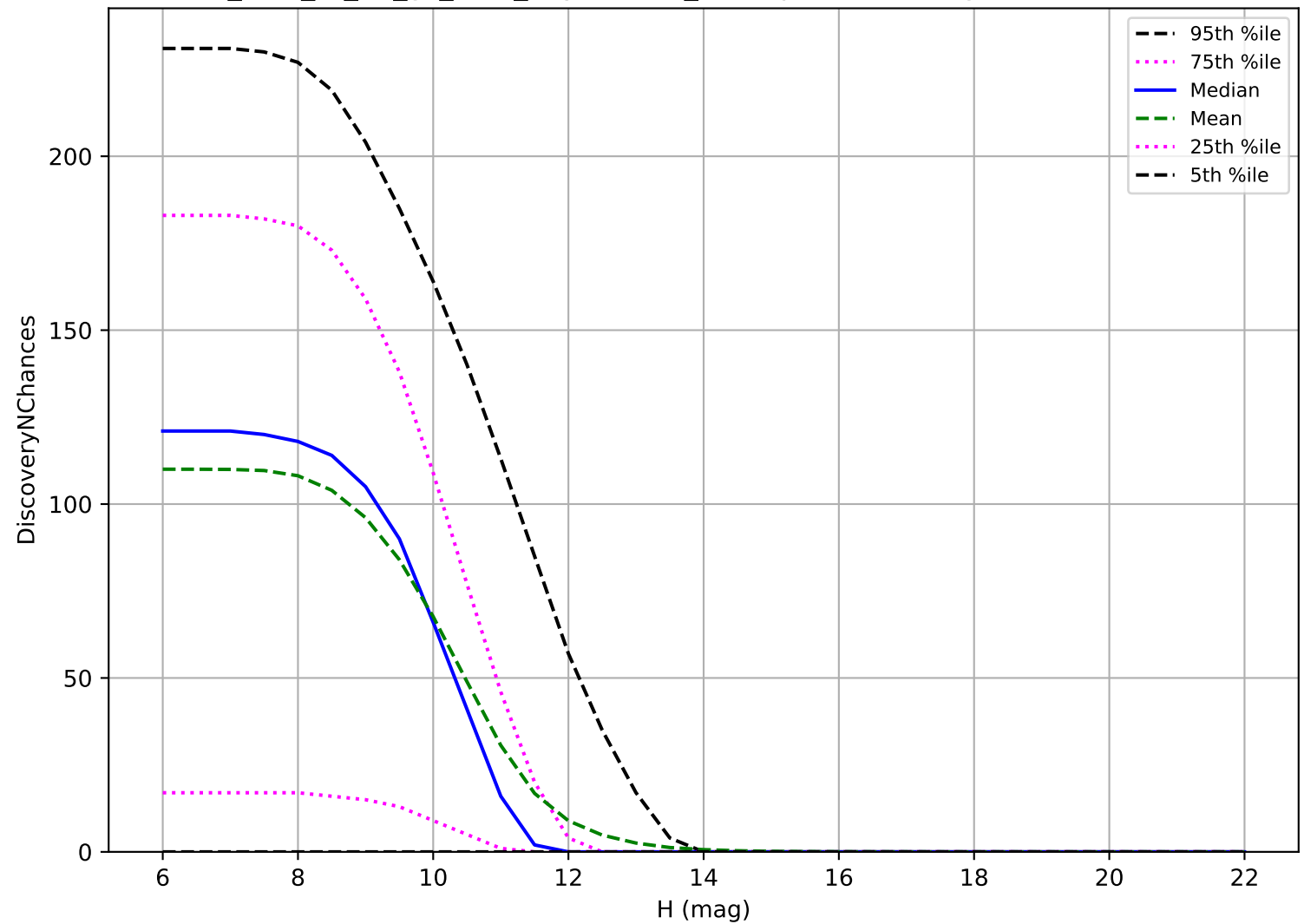
too_elab_r8_d3_gz_v3.4_10yrs: OCC_r20 3 pairs in 15 nights detection loss
