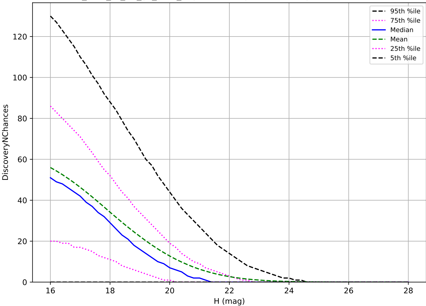
too_elab_r8_d3_gz_v3.4_10yrs: NEO 3 pairs in 15 nights detection loss
