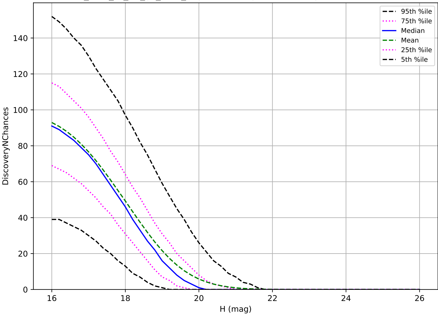
too_elab_r8_d3_gz_v3.4_10yrs: MBA 3 pairs in 15 nights detection loss
