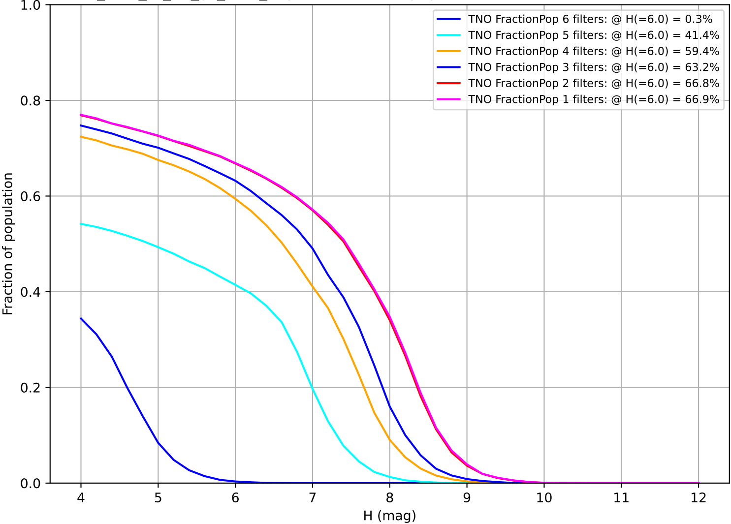
too_elab_r8_d3_gz_v3.4_10yrs: Fraction of population with colors in X filters TNO
