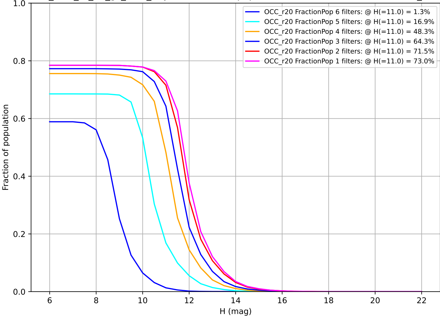
too_elab_r8_d3_gz_v3.4_10yrs: Fraction of population with colors in X filters OCC_r20
