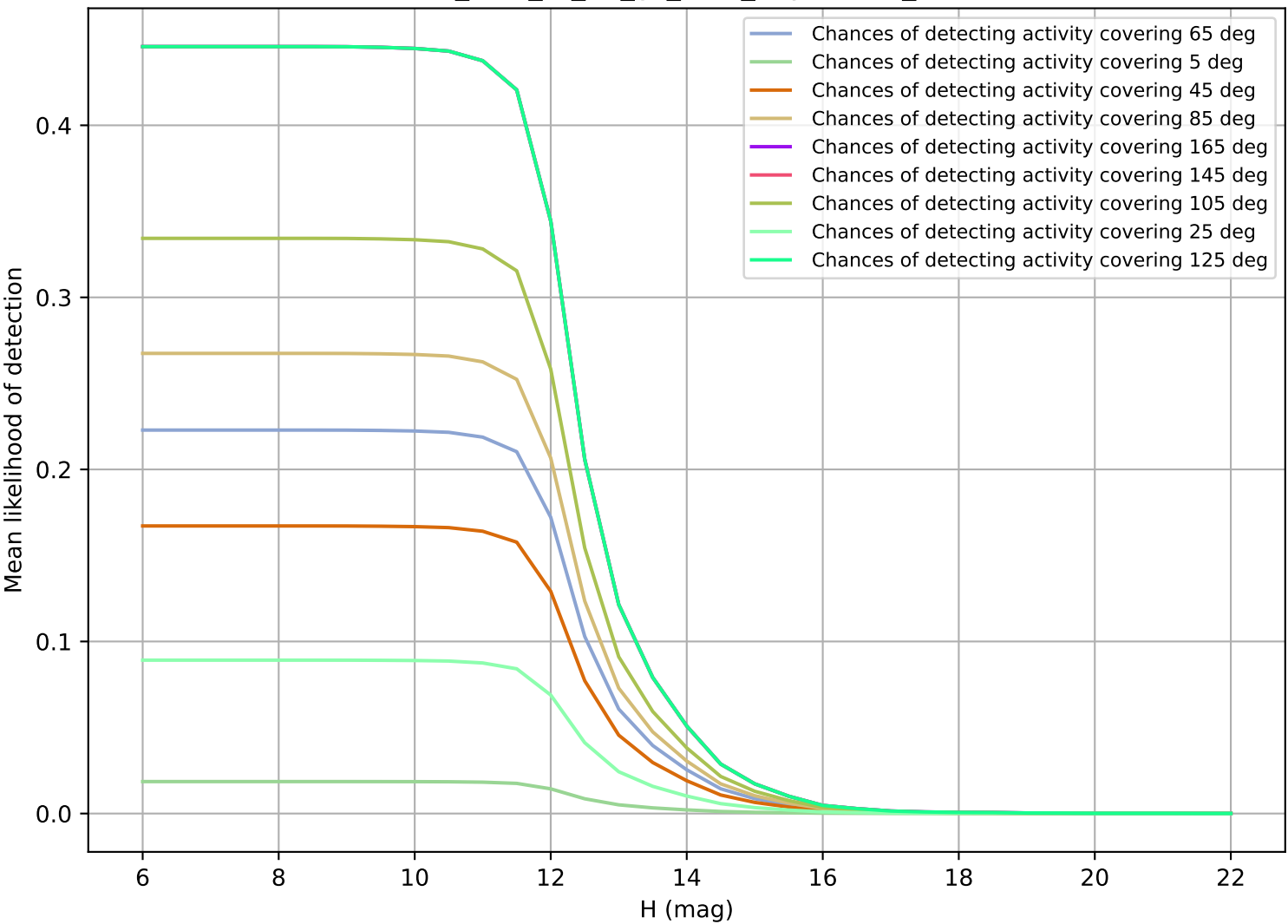
too_elab_r8_d3_gz_v3.4_10yrs OCC_r20
