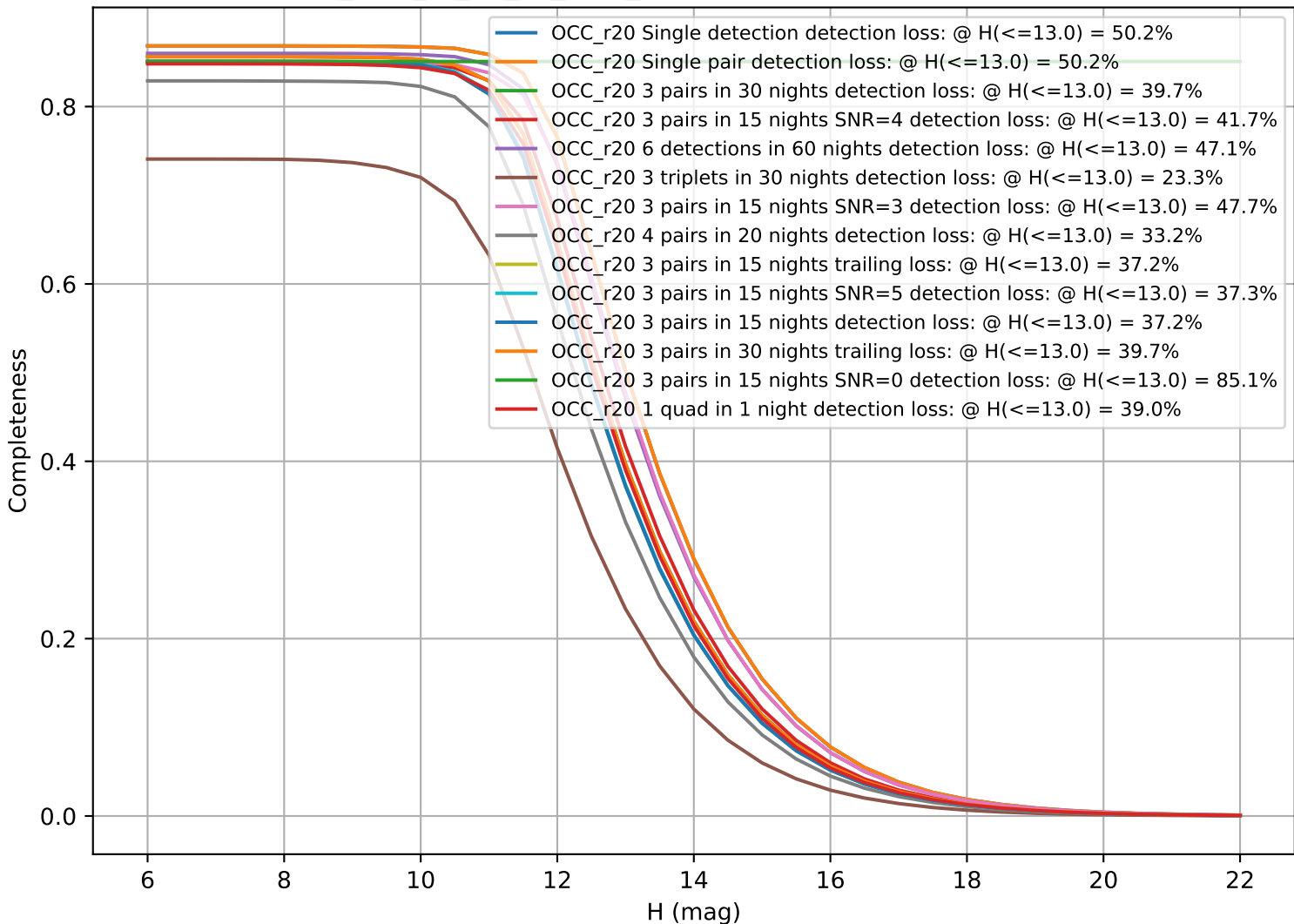
too_elab_r8_d3_gz_v3.4_10yrs: CumulativeCompleteness
