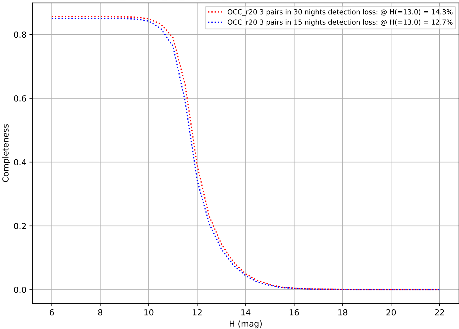
too_elab_r8_d3_gz_v3.4_10yrs: DifferentialCompleteness
